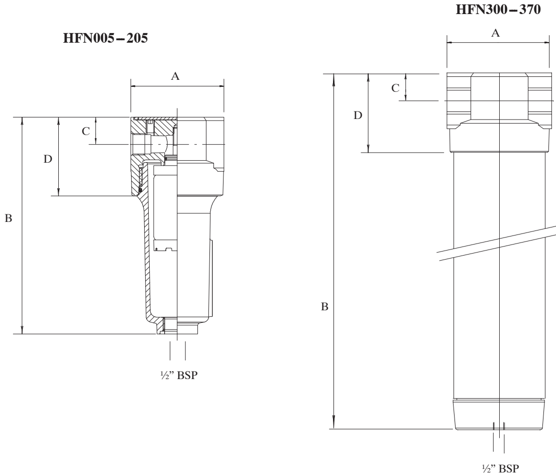
Fig.4 Overall dimensions
